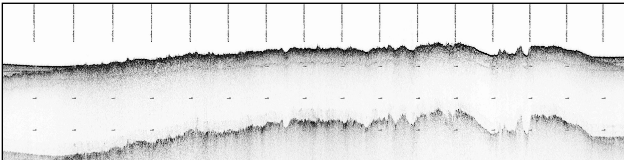
Fig. 13. Type D of seismo-acoustic facies (rocky).
