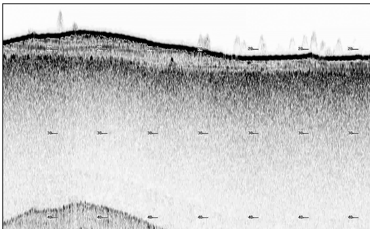
Fig. 10. Type A of seismo-acoustic facies.
