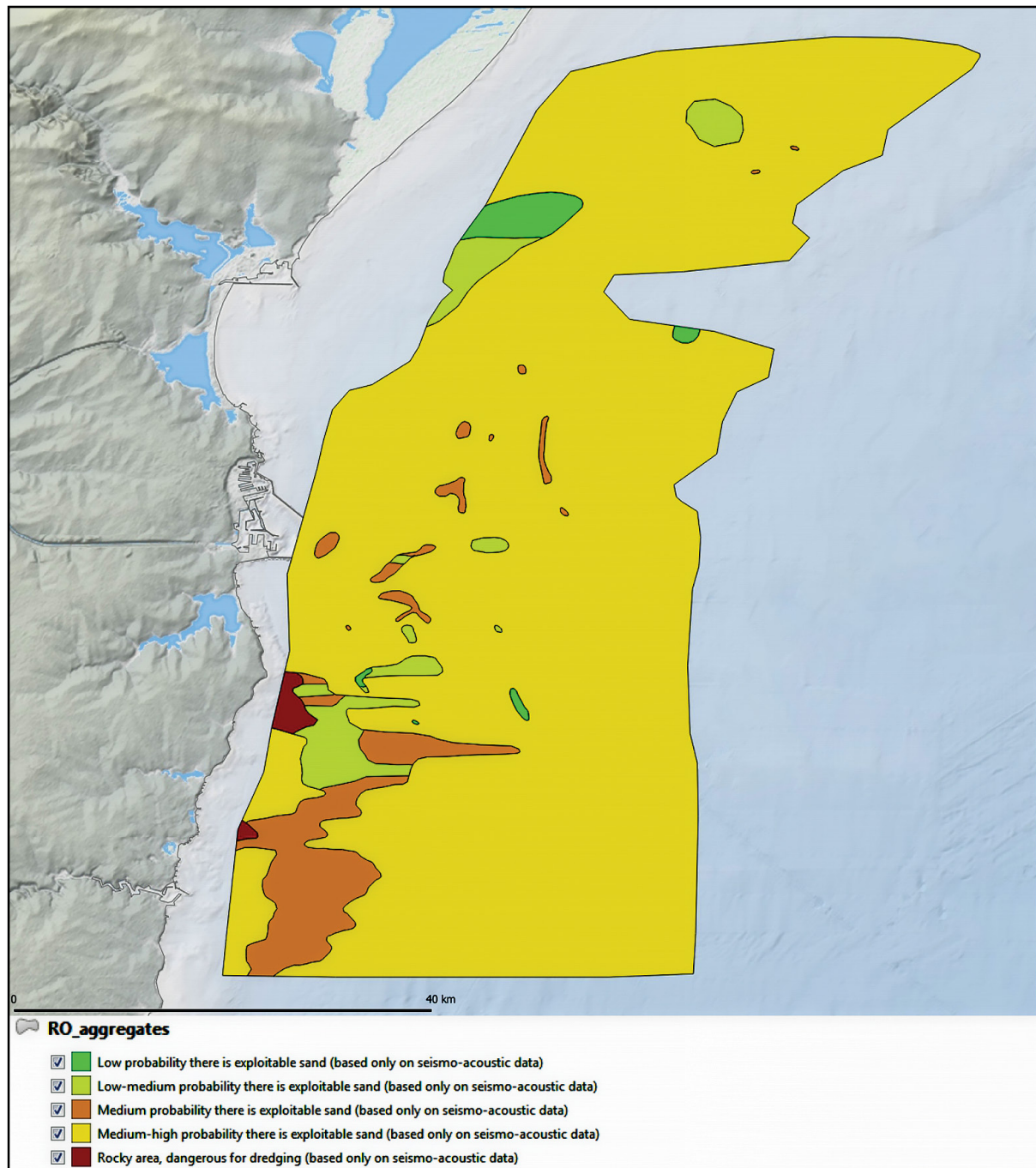
Fig. 14. Map of probability of offshore sand accumulations.
