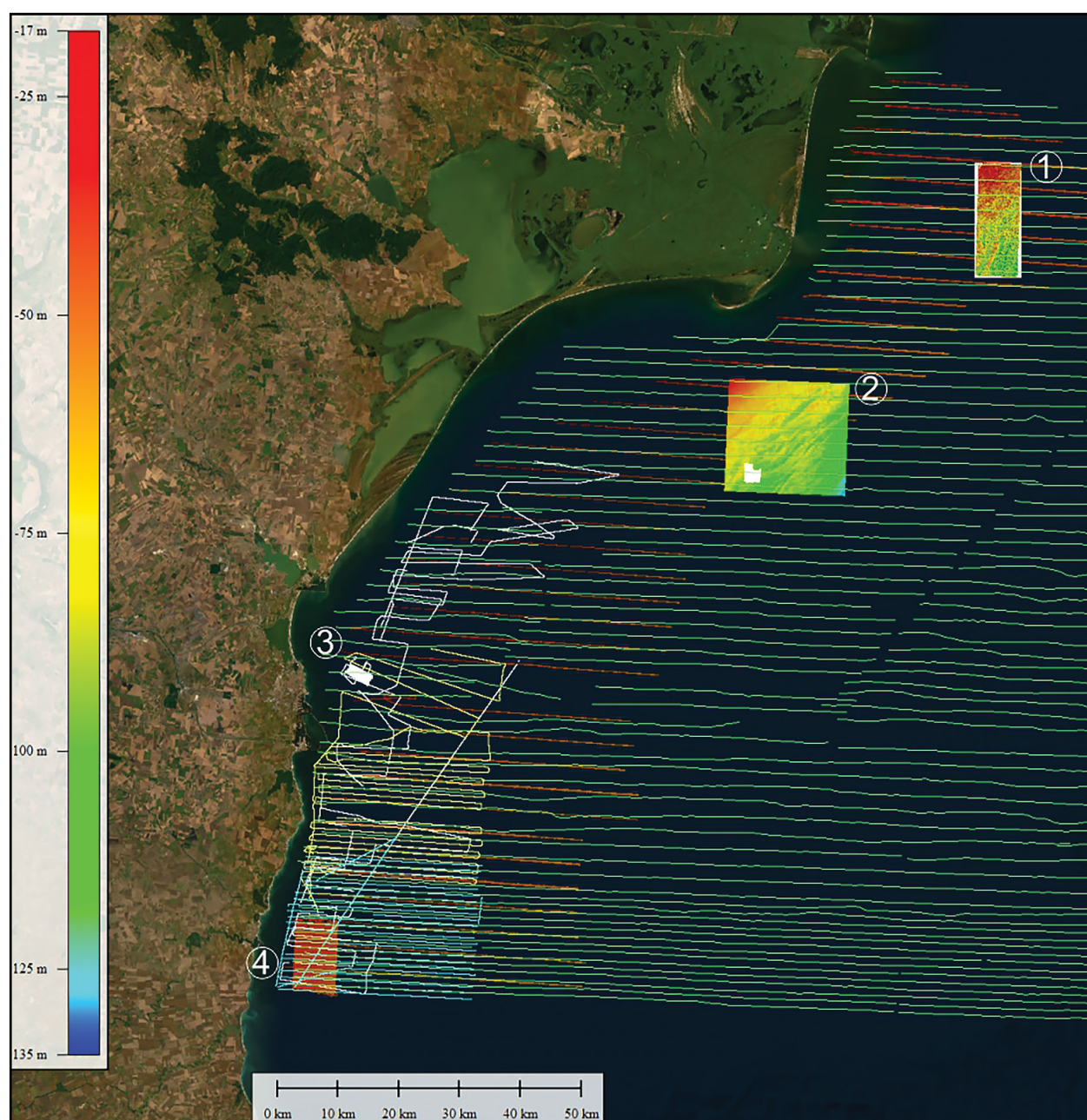
Fig. 4. Existing data in the area of interest (1, 2, 4 panels of DTM, 3 panel of DTM, SSS, and SBP): green lines – SBP 3.5 kHz; orange lines – MBES; yellow – MBES+SBP (chirp 2-12 kHz); cyan – MBES + SBP (chirp 2-12 kHz); white – MBES+SBP (chirp 2-12 kHz).
