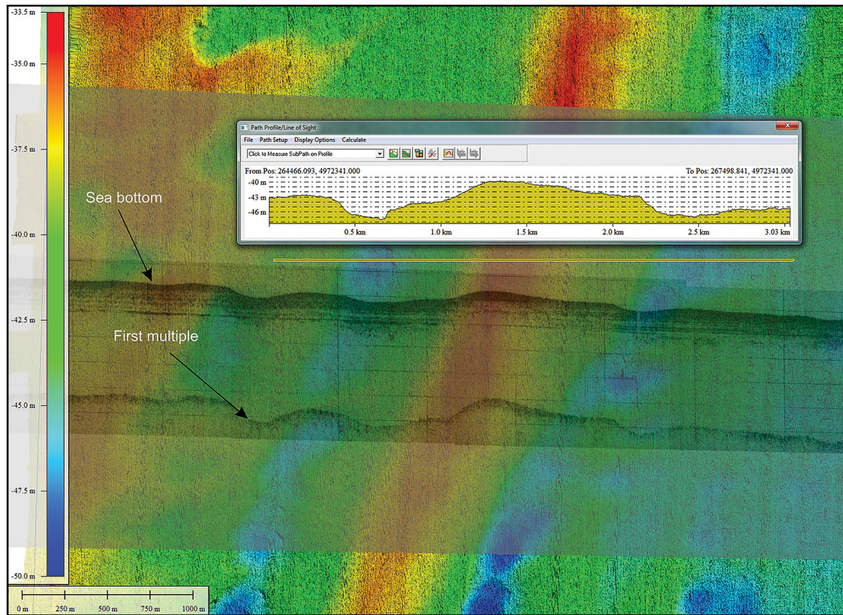
Fig. 5. Interpretation of MBES DTM and SBP data.
