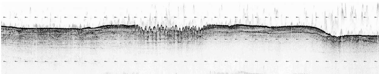
Fig. 9. Typical SBP seismo-acoustic facies for sand accumulations.
