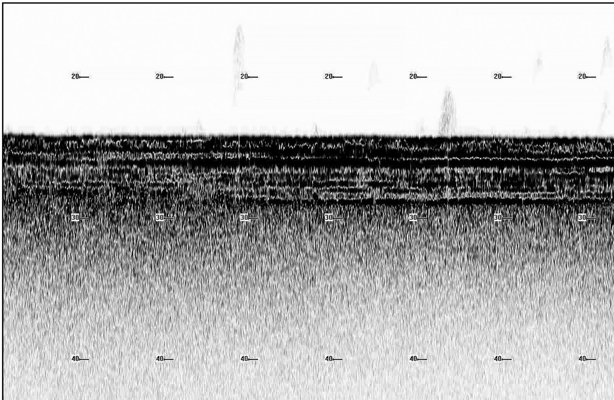
Fig. 12. Type C of seismo-acoustic facies.
