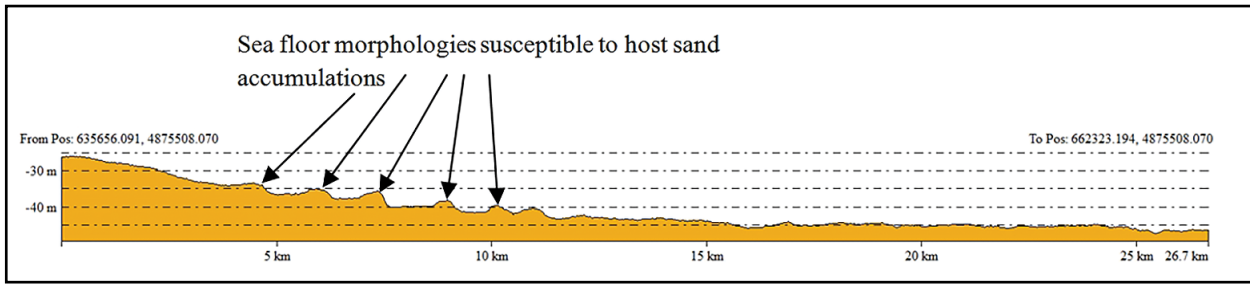
Fig. 7. DTM derived morphological profiles (after Ion et al. , 2020).
