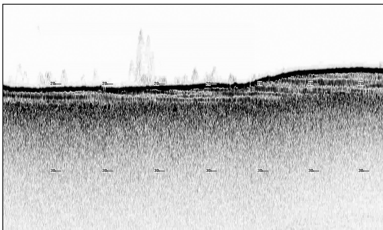
Fig. 11. Type B of seismo-acoustic facies.
