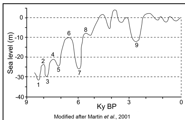
Fig. 1. Sea level variations curve.
