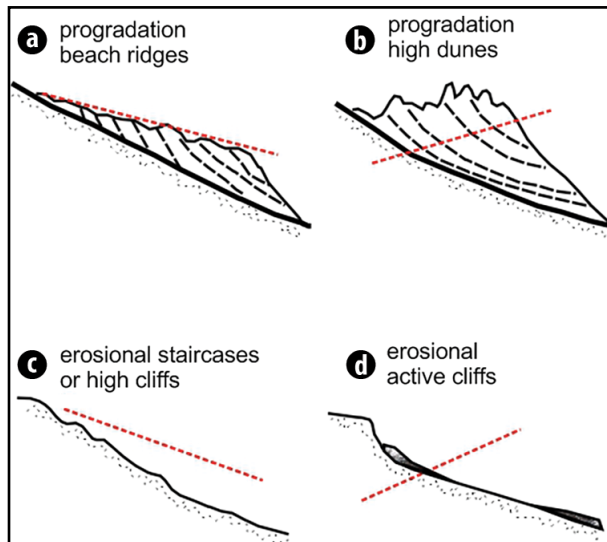
Fig. 3. Coastal development function of the relative sea level variation and availability of sediment a. falling sea level, high availability of sediment b. rising sea level, high availability of sediment c. falling sea level, scarce availability of sediment d. rising sea level, scarce availability of sediment (modified after Hansom, 2001).
