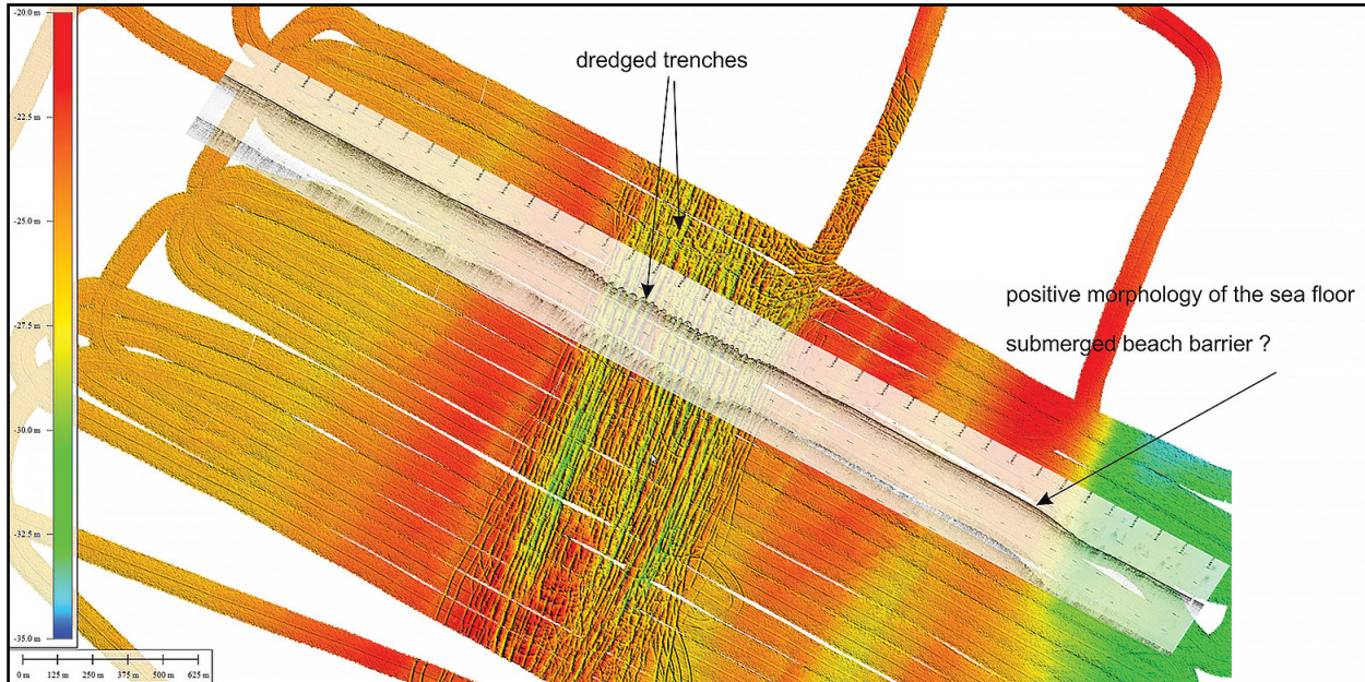
Fig. 8. Calibration of the seismo-acoustic facies on superimposed the images of DTM and SBP.
