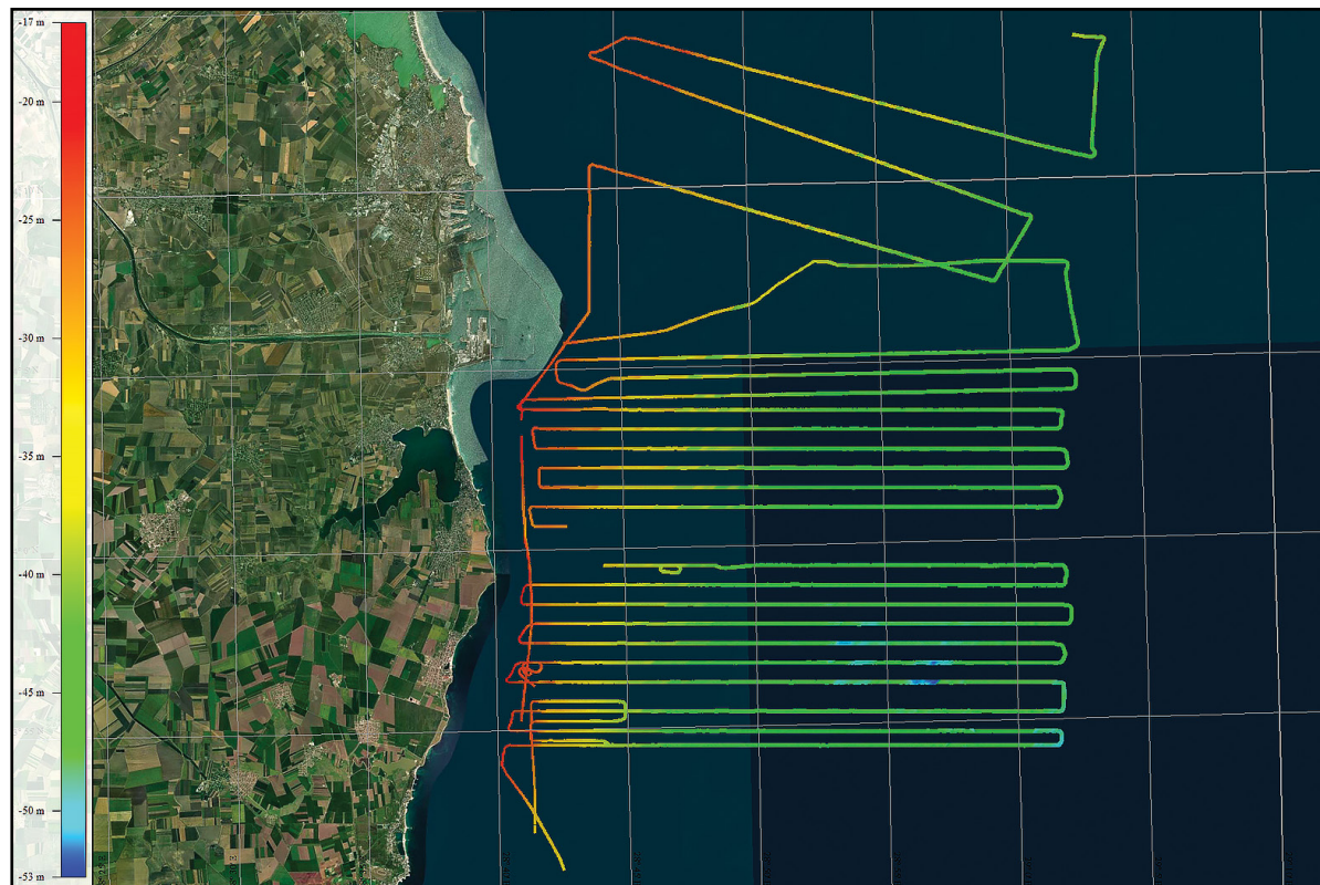
Fig. 6. Longitudinal along profile MBES DTMs, south of Constanta harbor (after Ion et al. , 2020).
